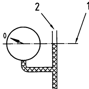
Figure 11 — Arrangement for determination of reference plane of spring pressure gauges
