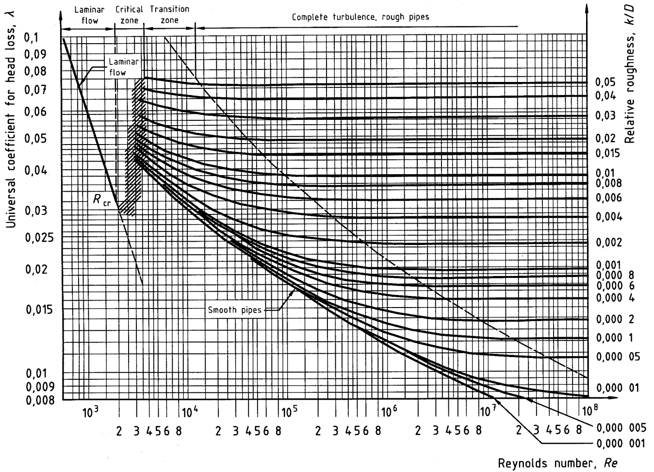
Figure C.4 — Values of universal coefficient for head loss (Moody chart)
