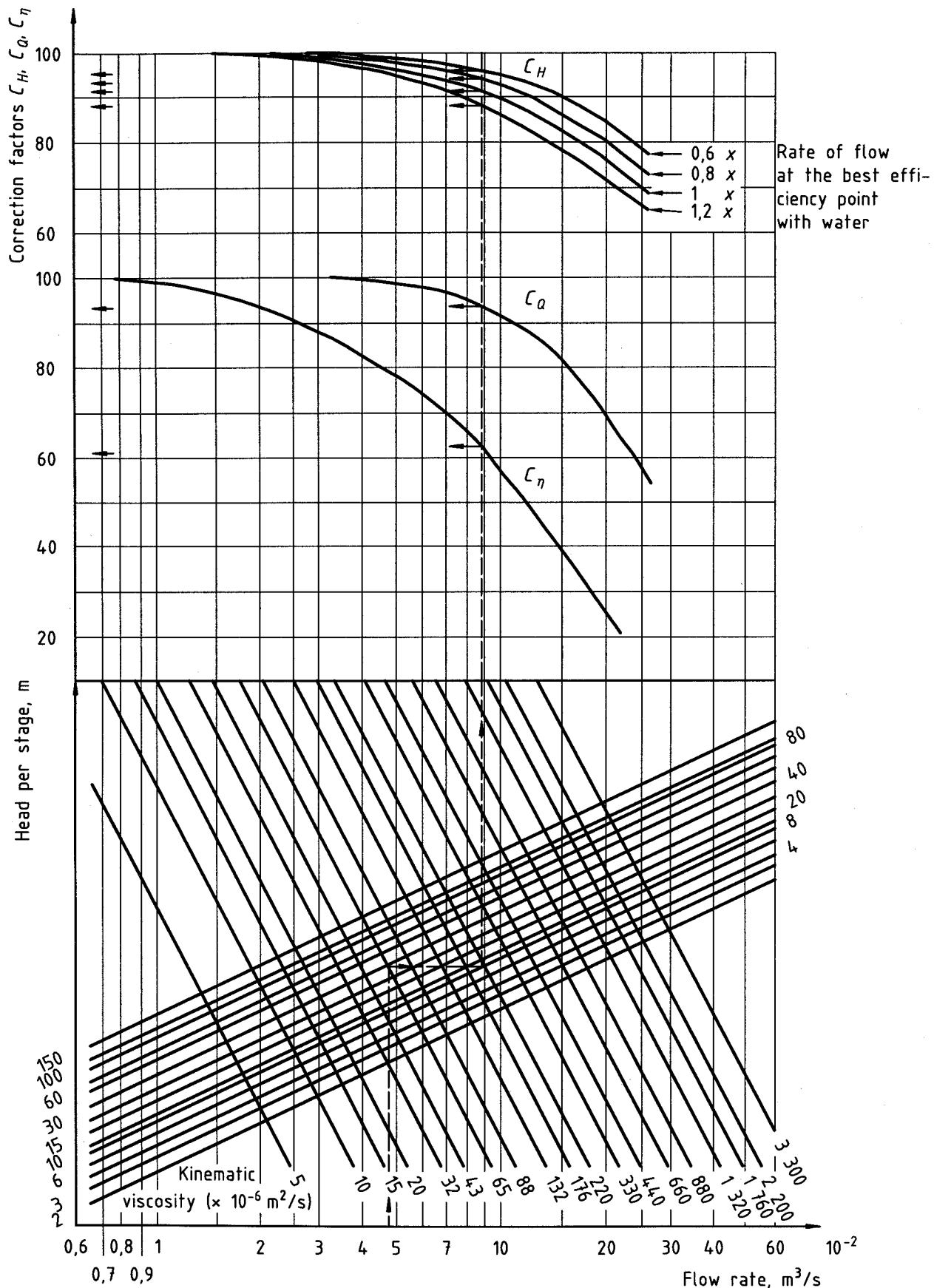
Figure G.1 — Performance correction chart for viscous liquids
