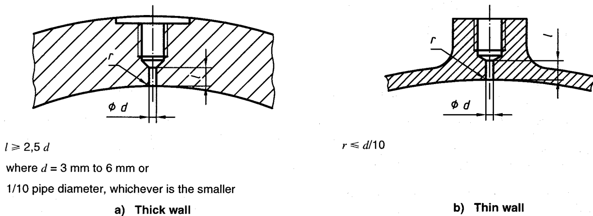
Figure 9 — Requirements for static pressure tapplings
