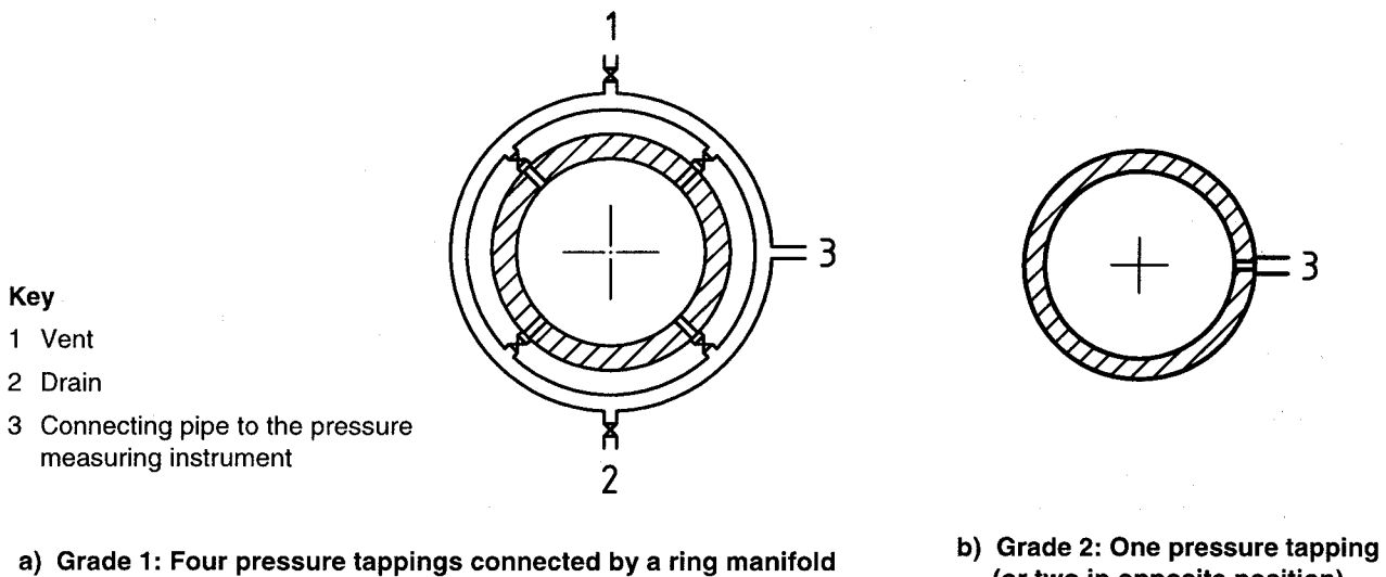
Figure 8 — Pressure tapping for grade 1 and 2 tests
