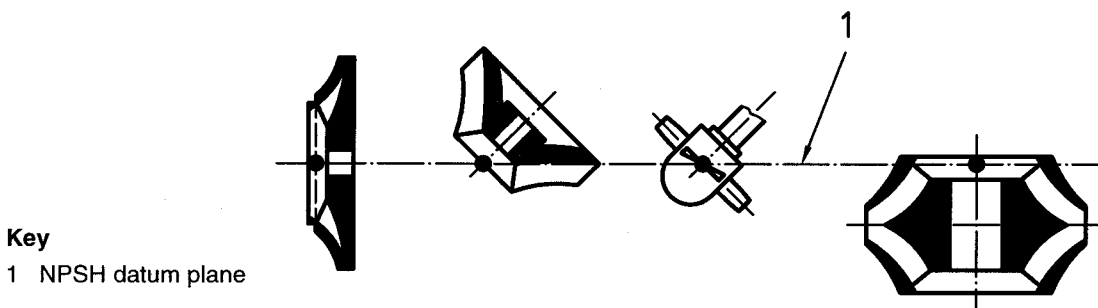
Figure 1 — NPSH datum plane
